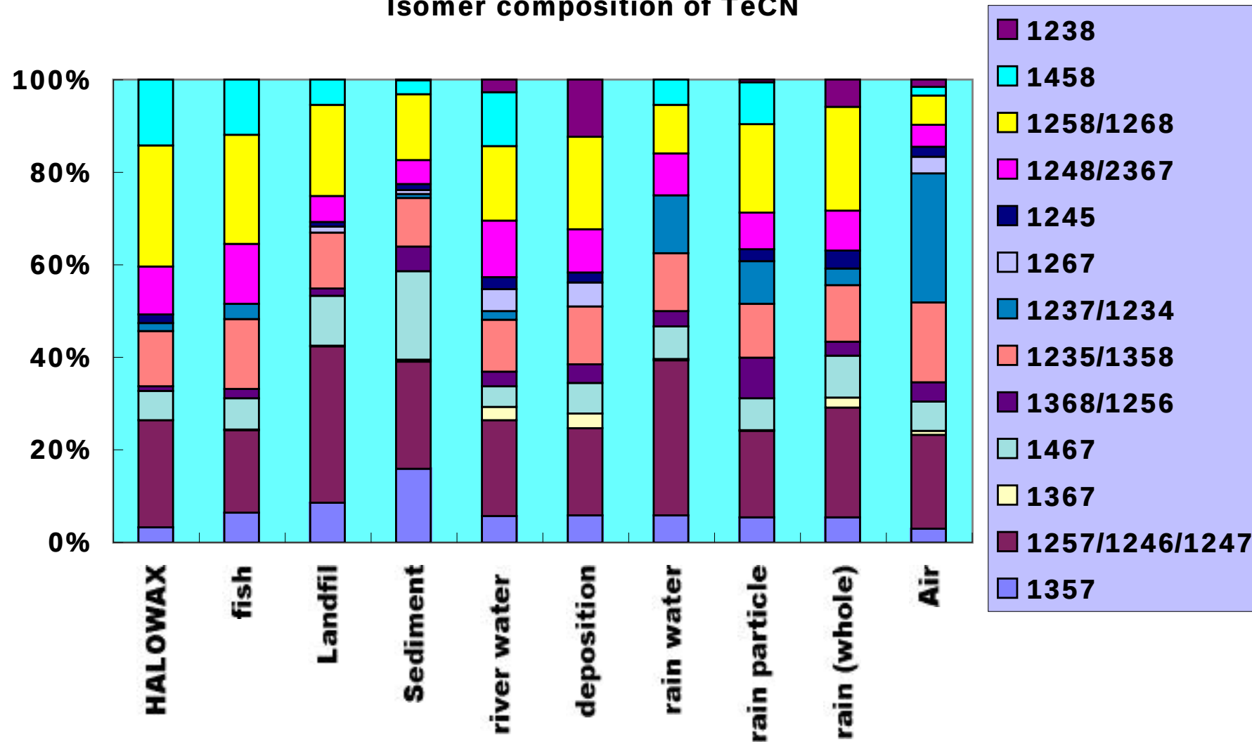
Isomer composition of TeCN
