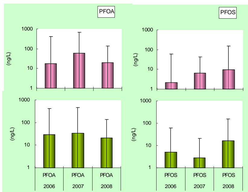
Figure4 Average of PFOA and PFOS concentrations(ng/L) in river water of Hyogo prefecture region from 2006 to 2008. Upper part is a graph calculated all samples. Under part is a graph calculated the 17 samples measuring 3 years in a row.
