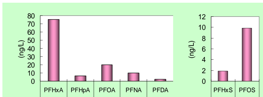
Figure2 Average of perfluorinated compounds concentrations(ng/L) in river water of Hyogo prefecture region in 2008. ( n=40, all samples)
