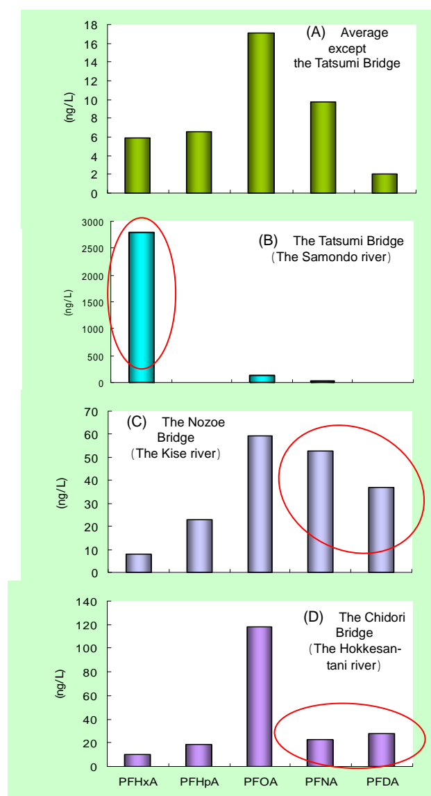
Figure3 Congener distribution of perfluorinated carboxylic acids (C6-C10) in river water of Hyogo prefecture region in 2008. (concentration unit is ng/L) (A) is a average graph calculated except the Tatsumi Bridge. (n=39) (B) is result of The Tatsumi Bridge (The Samondo river). (C) is result of The Nozoe Bridge (The Kise river). (D) is result of The Chidori Bridge (The Hokkesan-tani river).
